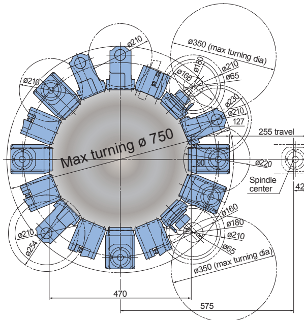
LT3000 (16) Position Multitasking Turret Interference Diagram
