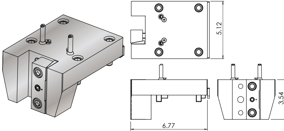
V760 / V920 • 2SP-V760 / 2SP-V920 OD-III Holder
